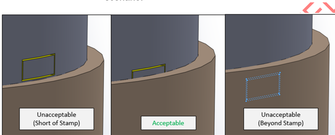
Figure 5: Acceptable / Unacceptable Make-up Positions
