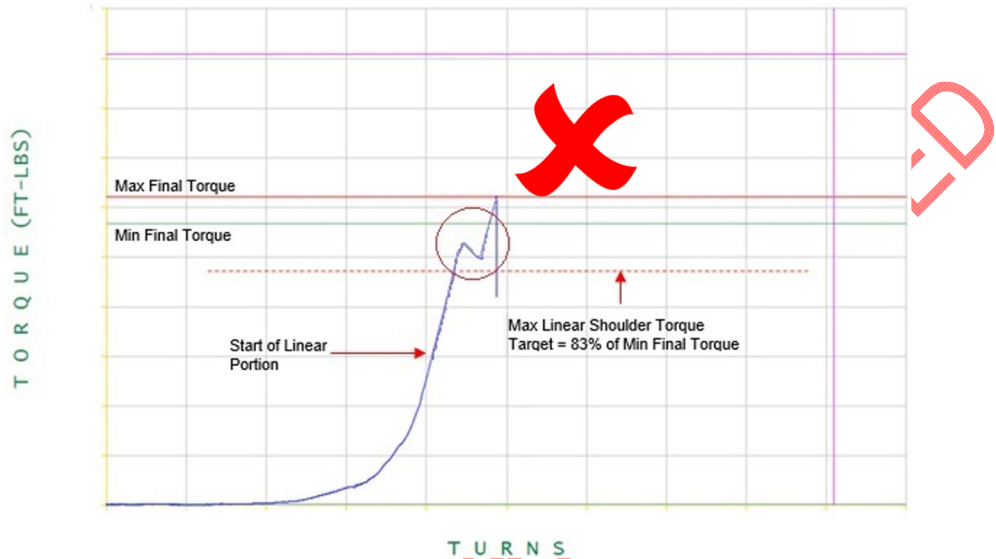
Figure 12: Unacceptable Linear Section to Final Torque
