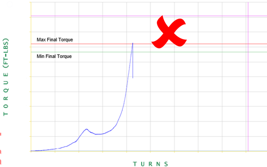
Figure 11: Irregularities in the Make-up Chart
