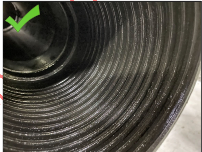
Figure 2: Example of 6.0" OD Proper Dope Amounts and Application
