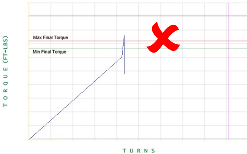
Figure 15: Irregularities in the make-up: Excessive initial torque build-up.
