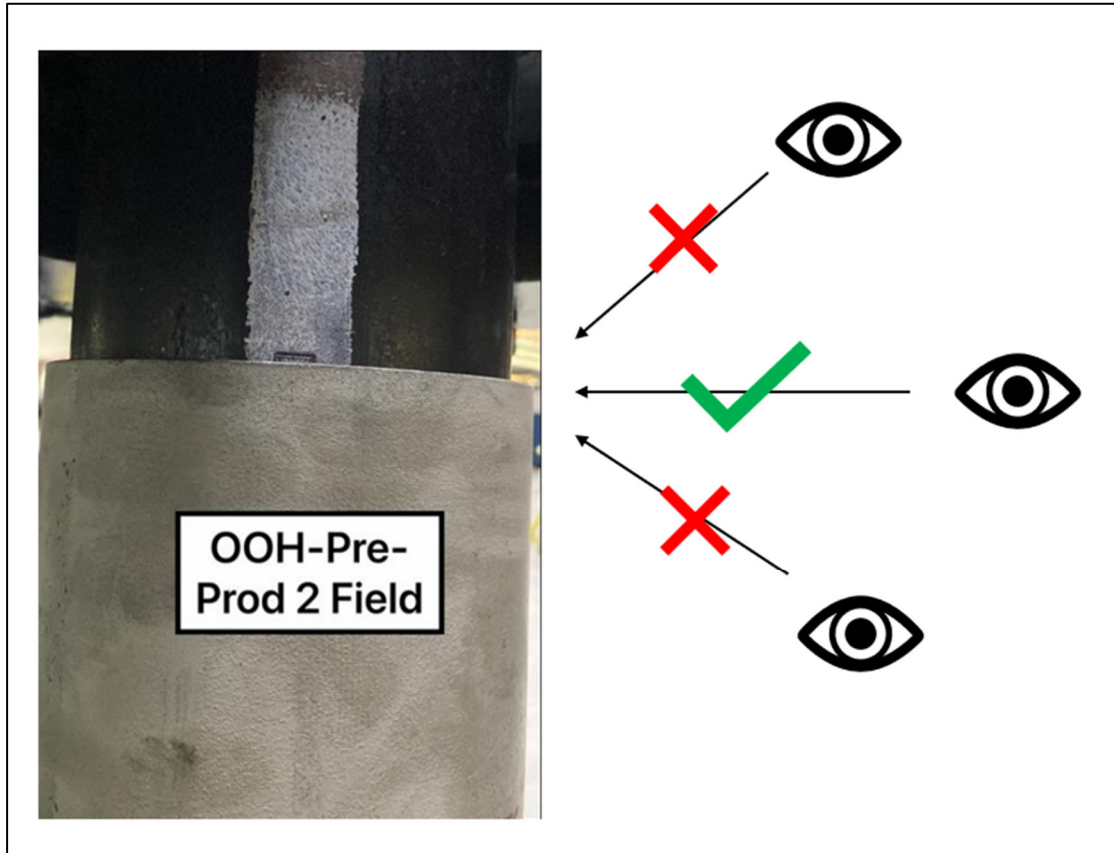
Figure 4: Acceptable Make-up Marker Viewing
