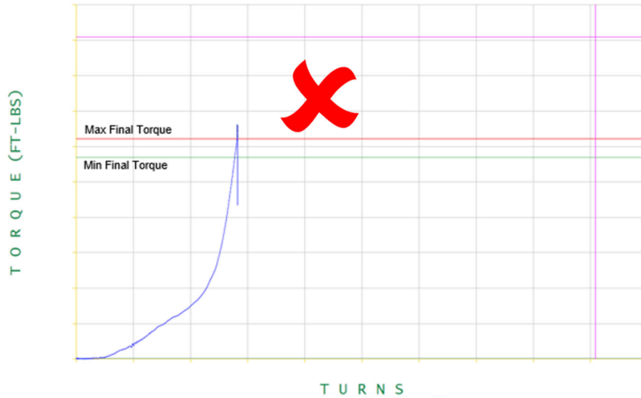
Figure 8: Exceeded Max Final Torque
