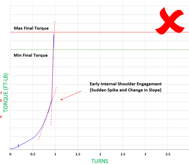
Figure 9: Early Internal Shoulder Engagement Prior to Final Torque
