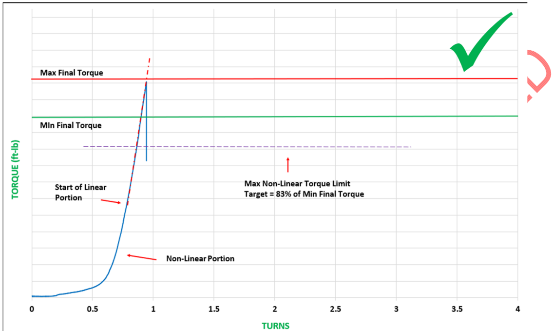
Figure 6: Typical Acceptable Make-up Signature
