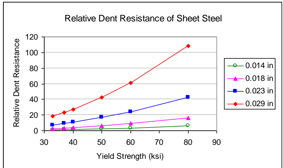
Figure 2. Relative dent resistance of sheet
